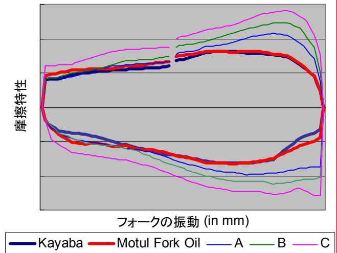
Motul Fork Oil と他社品の摩擦特性比較
